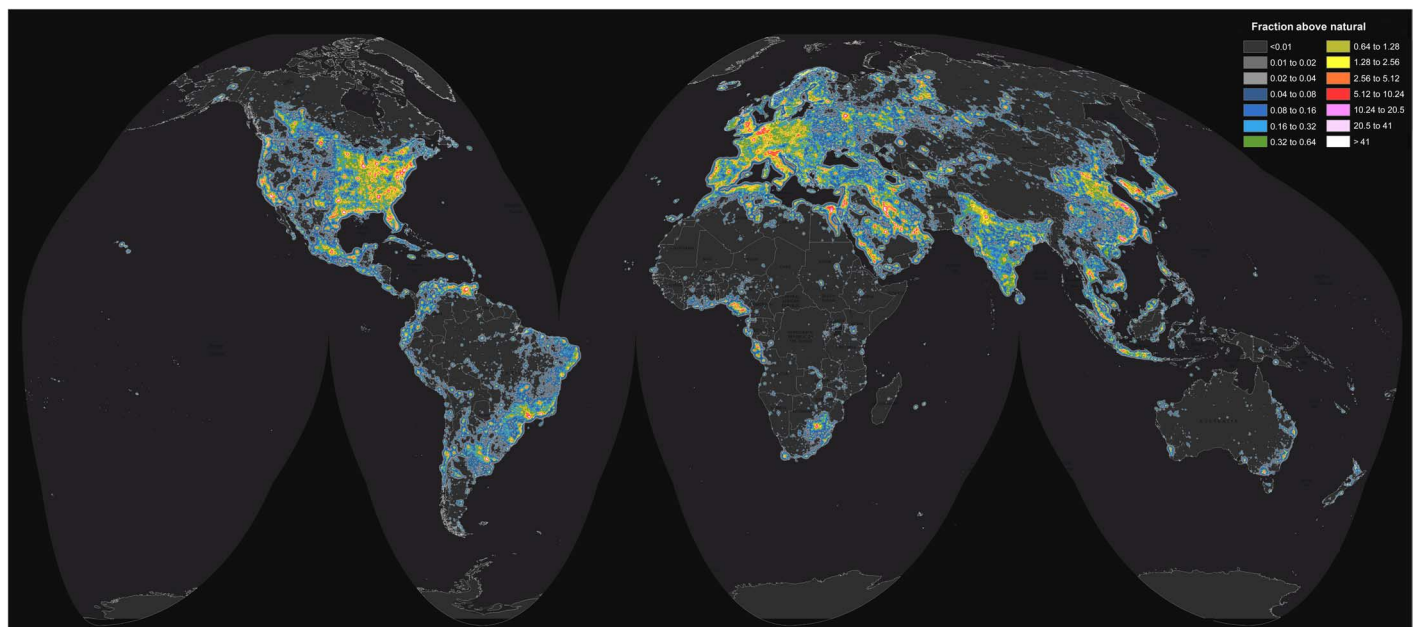
Fig. 2. World map of artificial sky brightness. The map shows, in twofold increasing steps, the artificial sky brightness as a ratio to the natural sky brightness (assumed to be 174 \text{ } \mu\text{cd/m}^2 ). Table 1 indicates the meaning of each color level.
